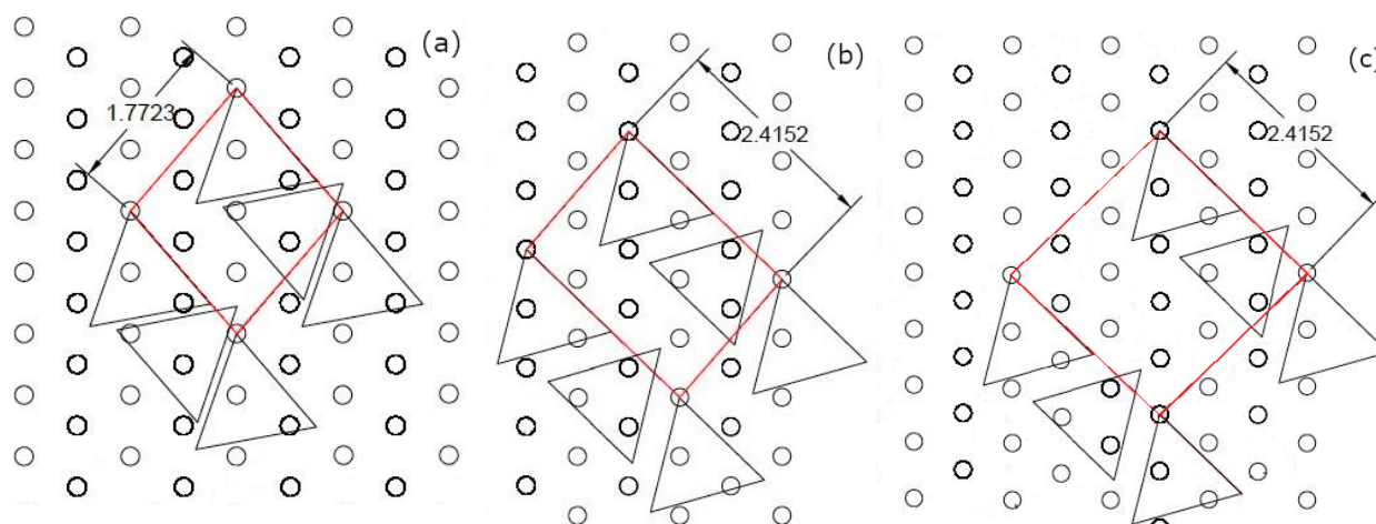
Figure 5.17. Three possible commensurate configurations with dimensions (a) 1.7723 \text{ nm} \times 1.7723 \text{ nm} , (b) 2.4152 \text{ nm} \times 1.7723 \text{ nm} and (c) 2.4152 \text{ nm} \times 2.4152 \text{ nm} . Dots represent the \sqrt{3} lattice points.
