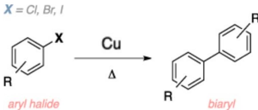
Figure 2. 14. Coupling reaction involving two aryl halides with a copper catalyst. Figure reproduced from Ullmann et al. (1901)
