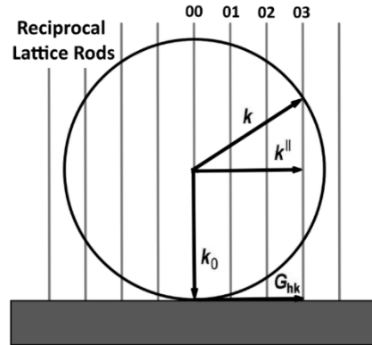
Figure 3.5. The Ewald sphere within the 2-d reciprocal lattice.
