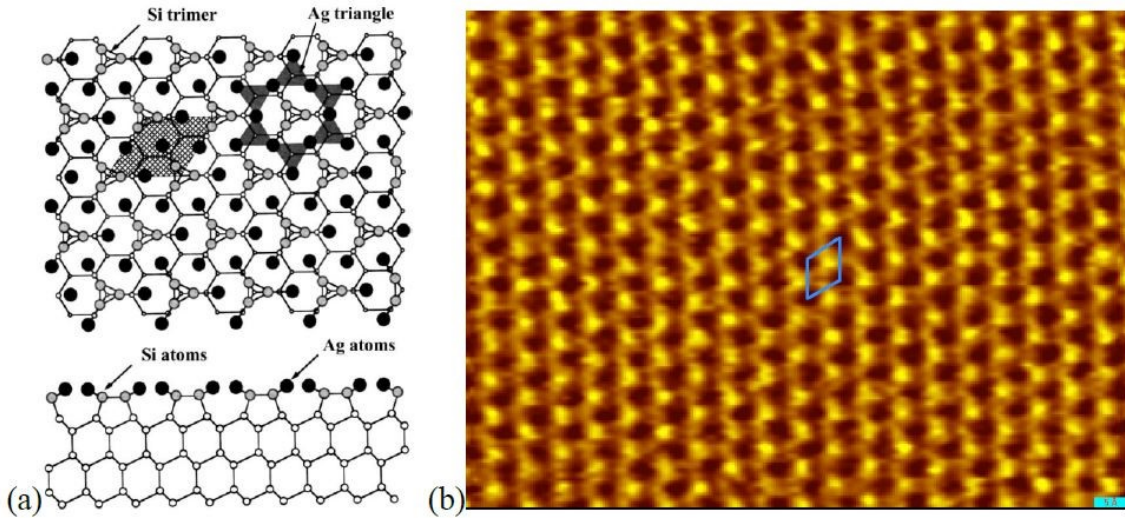
Figure 2. 6. (a) The atomic structure of the \sqrt{3} -Ag reconstruction, with the hexagonal unit cell shaded. Figure reproduced from Tong et al. (2002). (b) A 100Å×100Å STM image of the \sqrt{3} -Ag surface with unit cell highlighted in blue.
