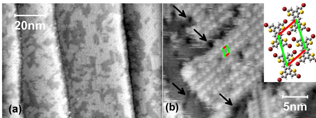
Figure 4.5. STM images of TBTTA superstructures on the \sqrt{3} surface ( V_{\text{sample}} = -1.11 V, I = 0.5 nA). The image in (a) reveals four TBTTA-covered \sqrt{3} terraces separated by single height Si atomic steps running vertically in the image. The zoomed-in image (b) highlights both the unit cell and defects in the \sqrt{3} structure (arrows), which appear to limit the extent of the TBTTA domain.
