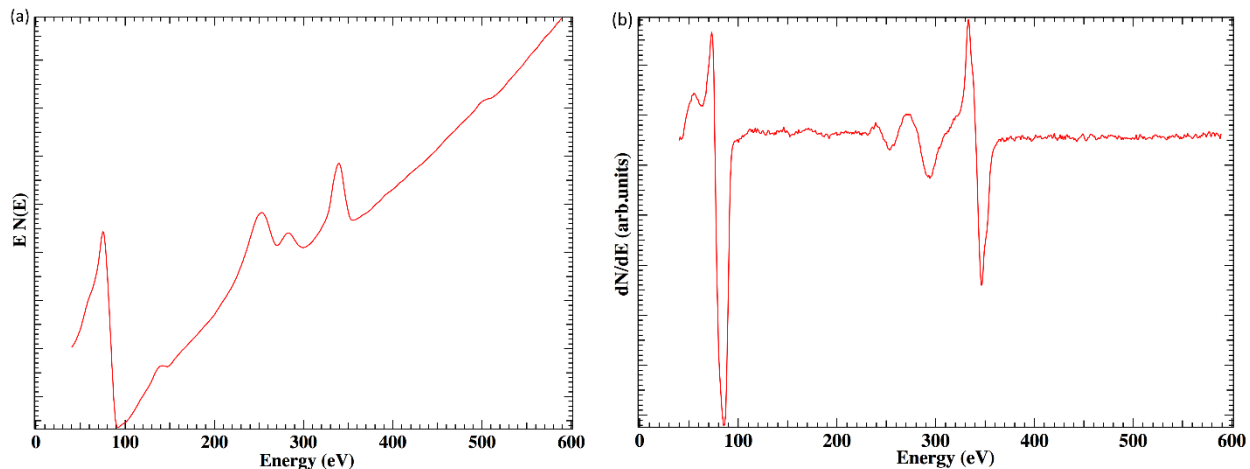
Figure 3.10. An Auger spectrum for one monolayer of Ag on Si(111) plotted as (a) intensity vs. energy and (b) the derivative dN/dE vs. energy.
