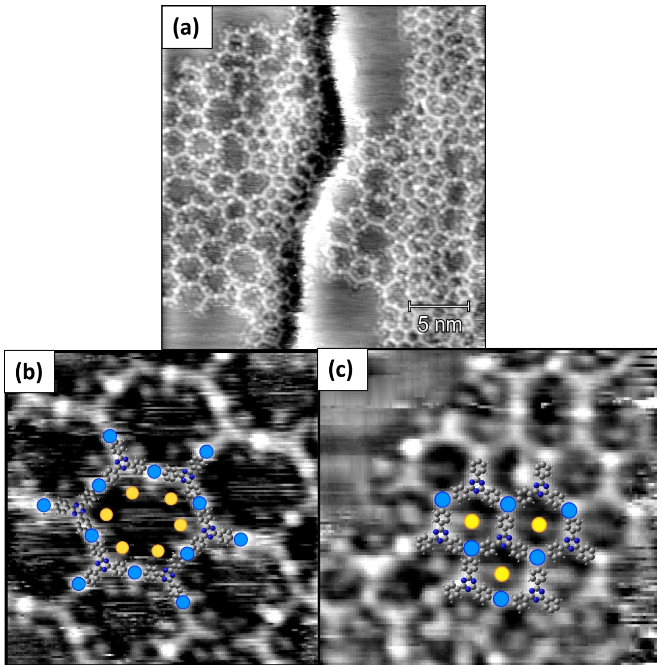
Figure 5.6. (a) A large scan of the organometallic structures of TIPT on Ag(111). (b) A zoomed in image of the organometallic structures. Silver adatoms and iodine atoms are pointed by blue and yellow dots respectively. (c) A region in which one silver adatom is coordinated to three radicals. Single iodine atom is also observed inside the pore.
